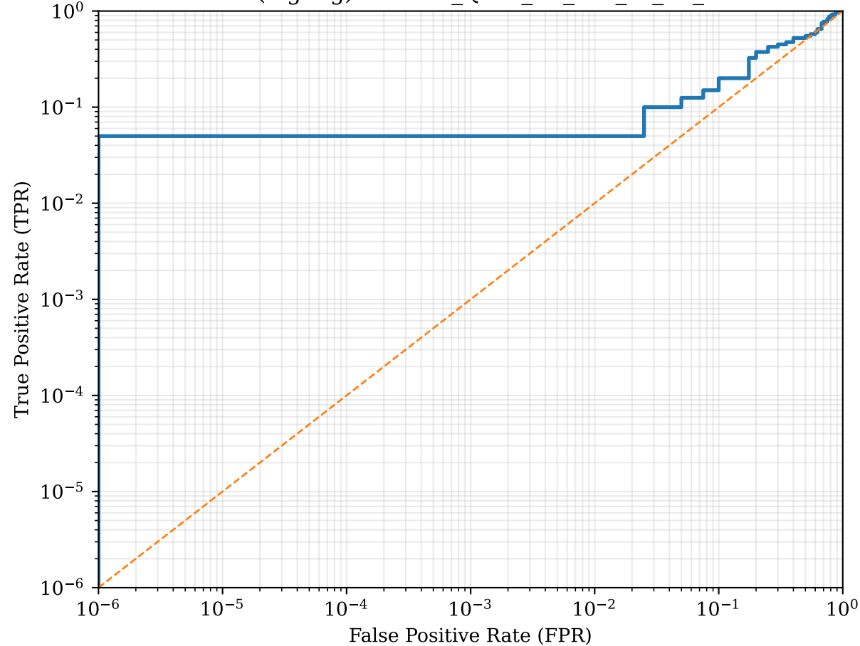
ROC (log-log): MNIST_QNN_eff_su2_r5_d6_s43
