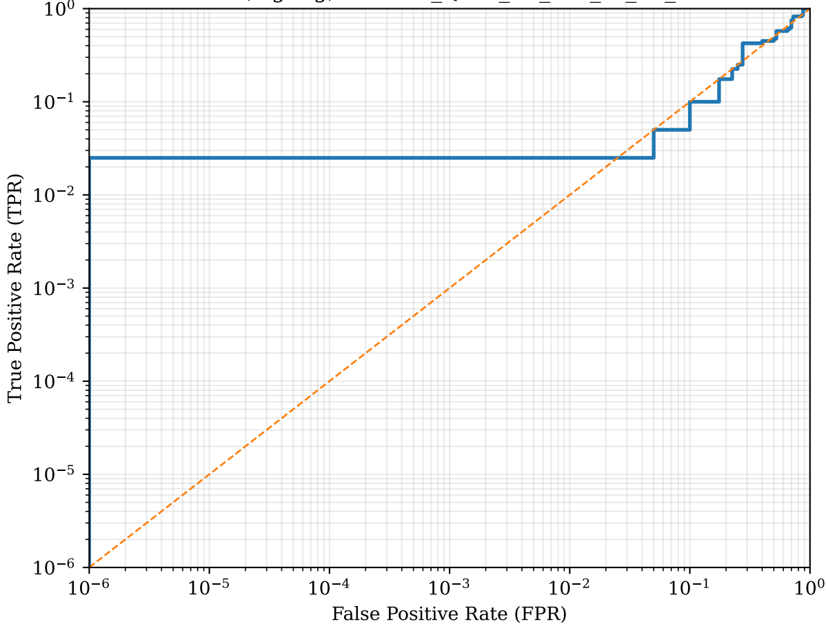
ROC (log-log): MNIST_QNN_eff_su2_r5_d6_s45
