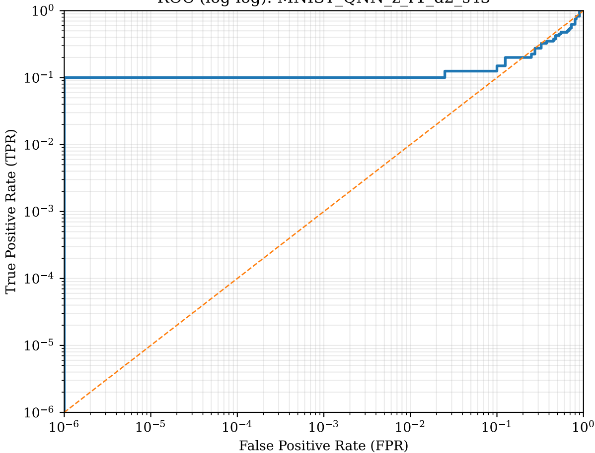
ROC (log-log): MNIST_QNN_z_r1_d2_s43
