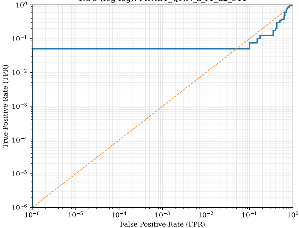
ROC (log-log): MNIST_QNN_z_r1_d2_s44
