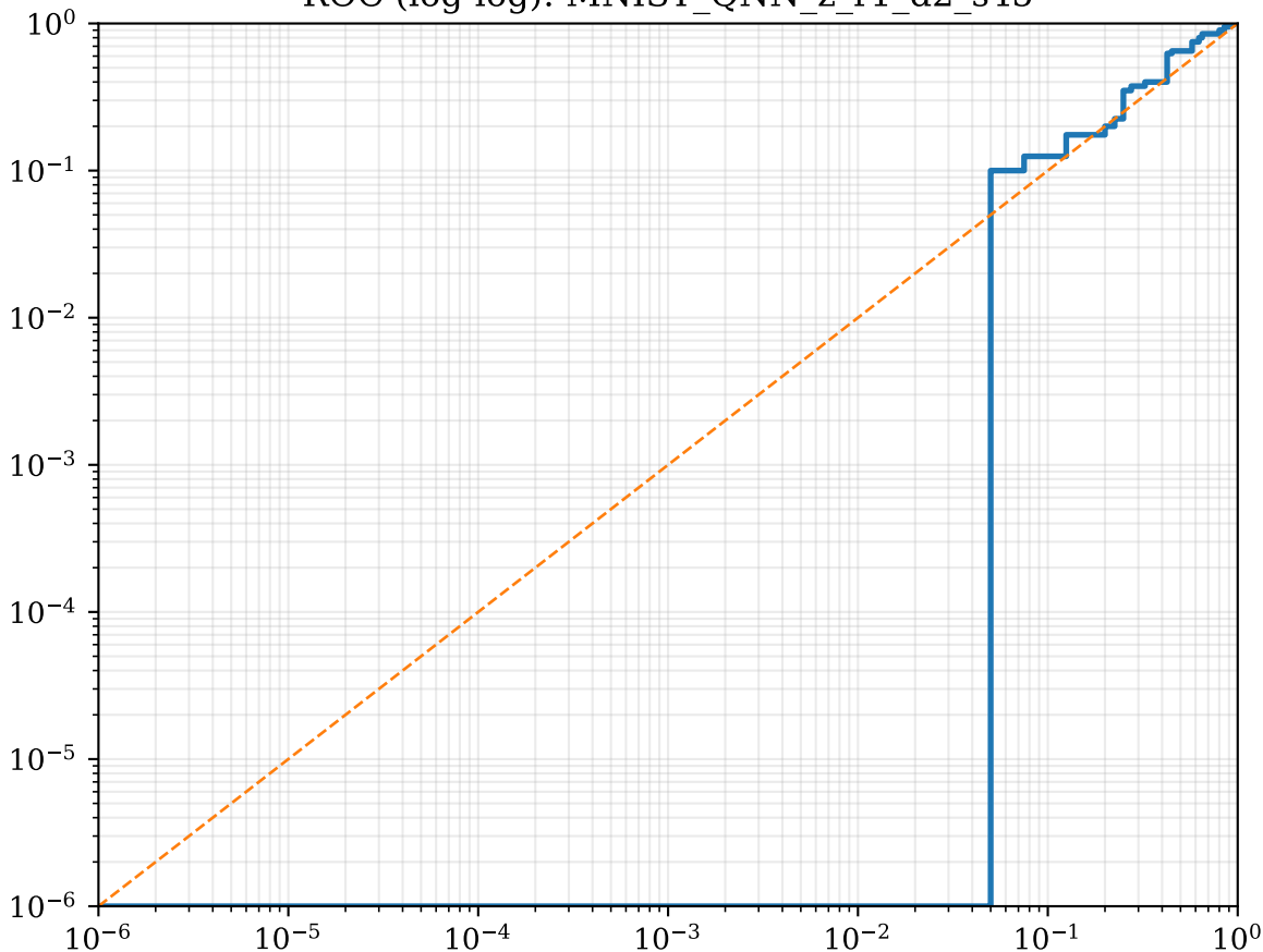
ROC (log-log): MNIST_QNN_z_r1_d2_s45
