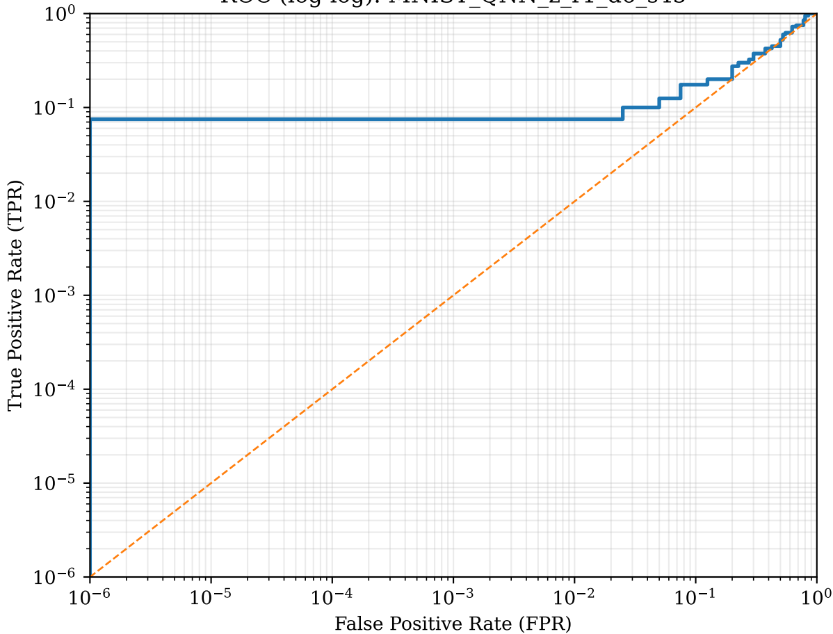
ROC (log-log): MNIST_QNN_z_r1_d6_s45
