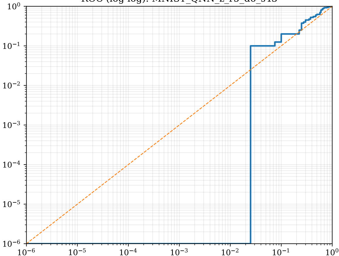
ROC (log-log): MNIST_QNN_z_r5_d6_s43
