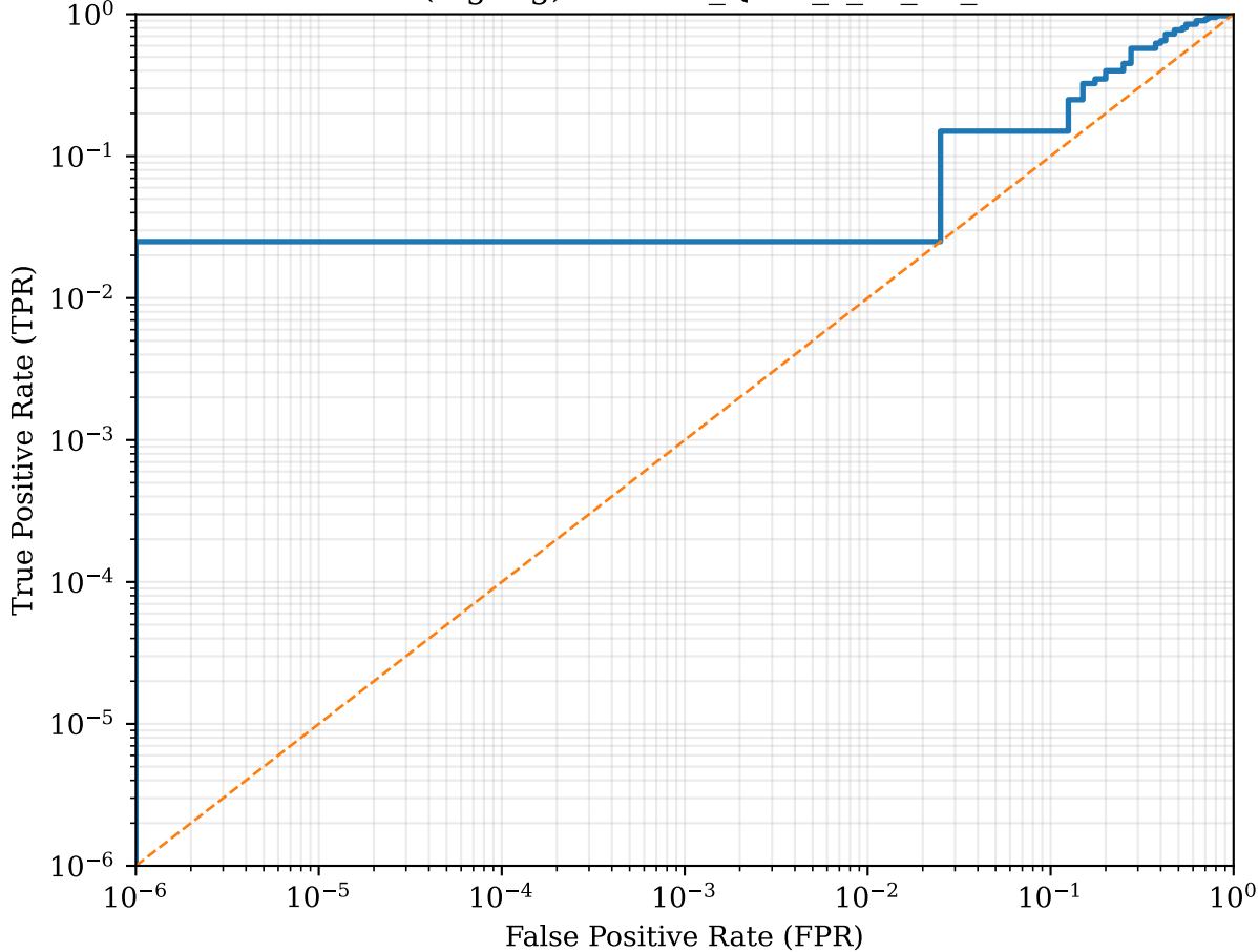
ROC (log-log): MNIST_QNN_z_r5_d6_s44
