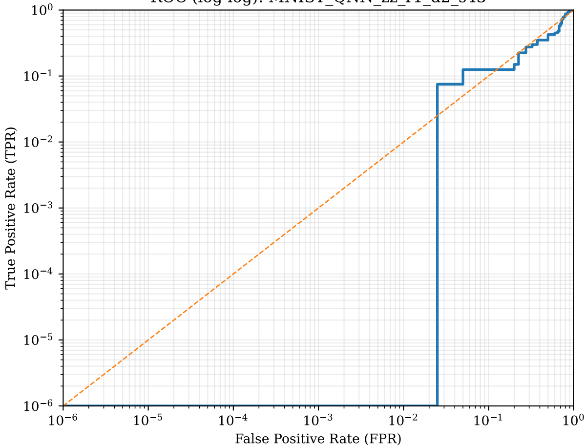
ROC (log-log): MNIST_QNN_zz_r1_d2_s43
