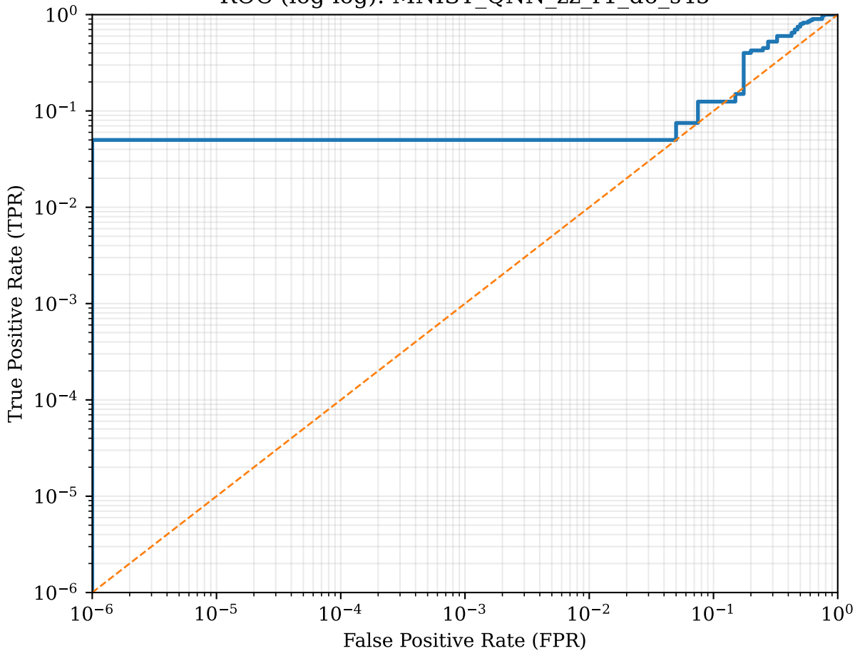
ROC (log-log): MNIST_QNN_zz_r1_d6_s45
