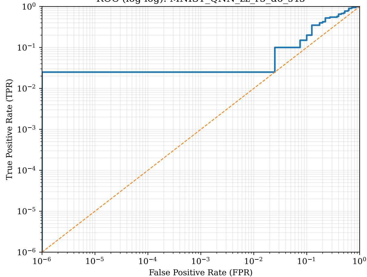
ROC (log-log): MNIST_QNN_zz_r5_d6_s45
