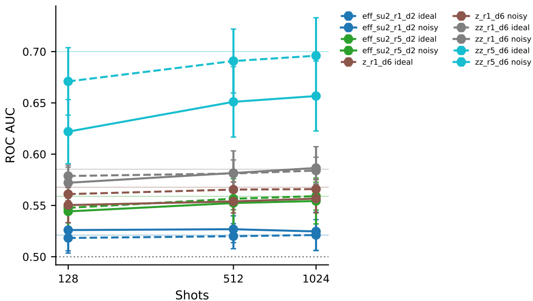
Loss-threshold MIA
