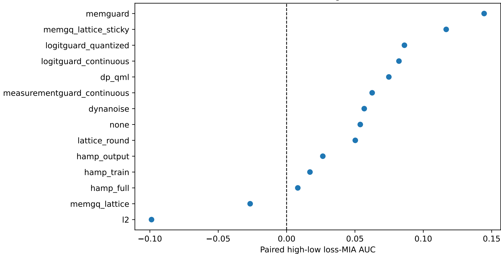
Residual structural leakage under defense
