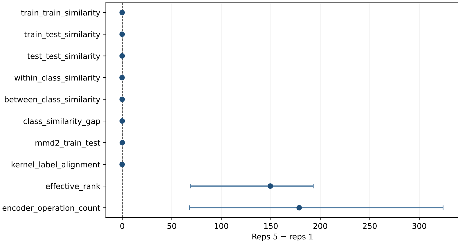
FASHION repetition-induced geometry changes
