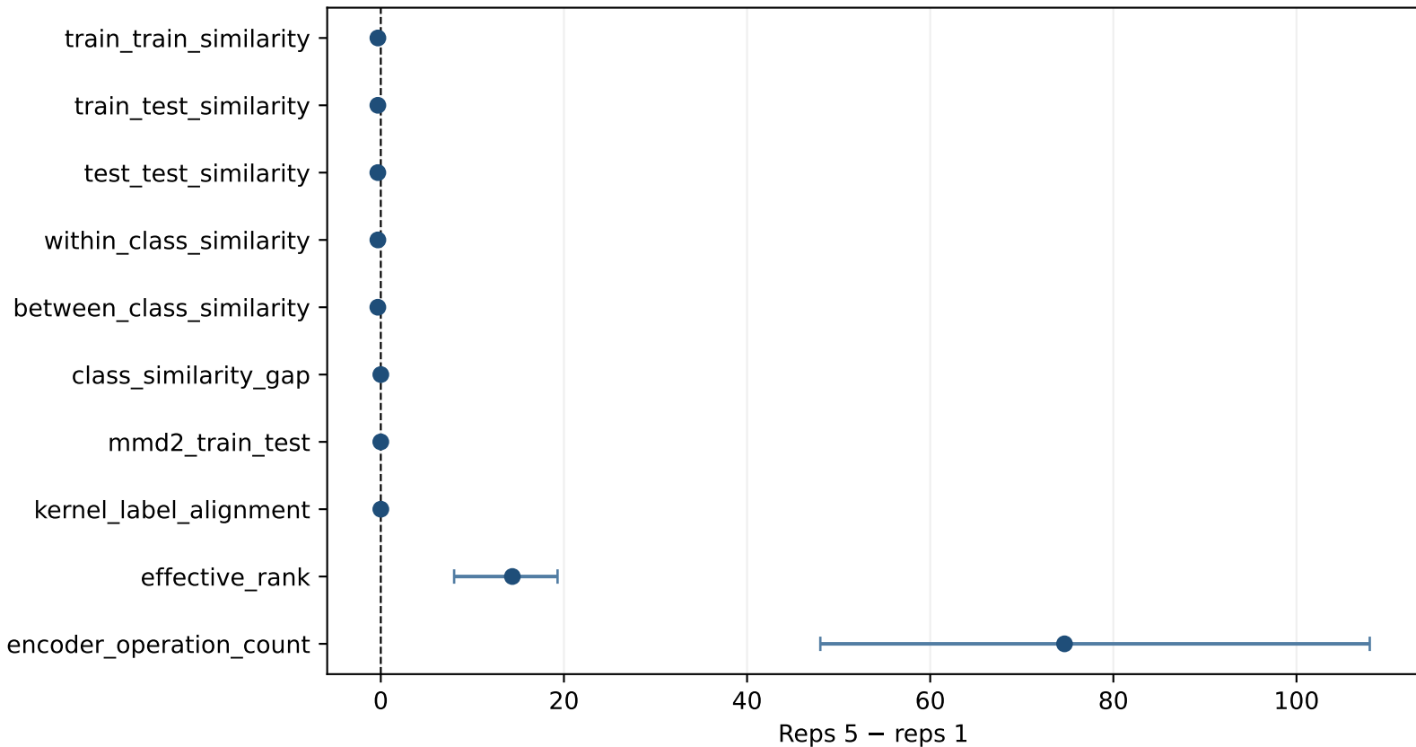
Repetition-induced post-encoder geometry changes
