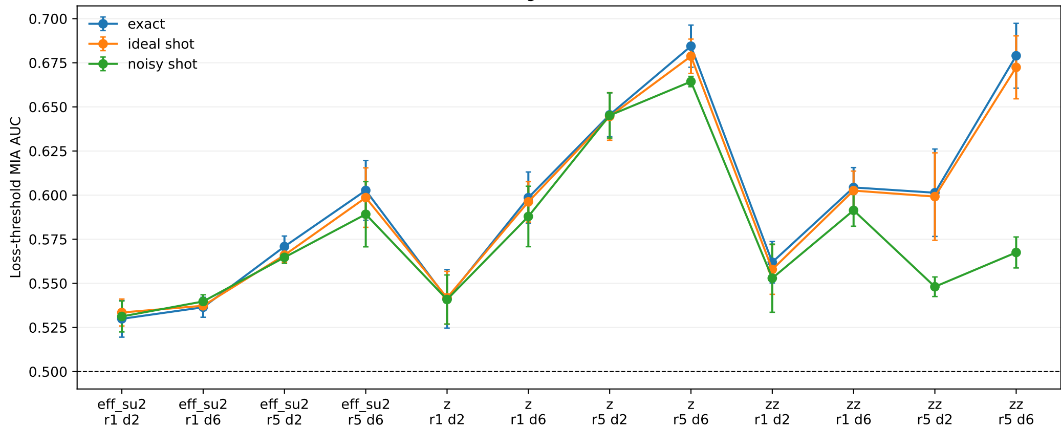
N1 structural ordering under frozen finite-shot noise
