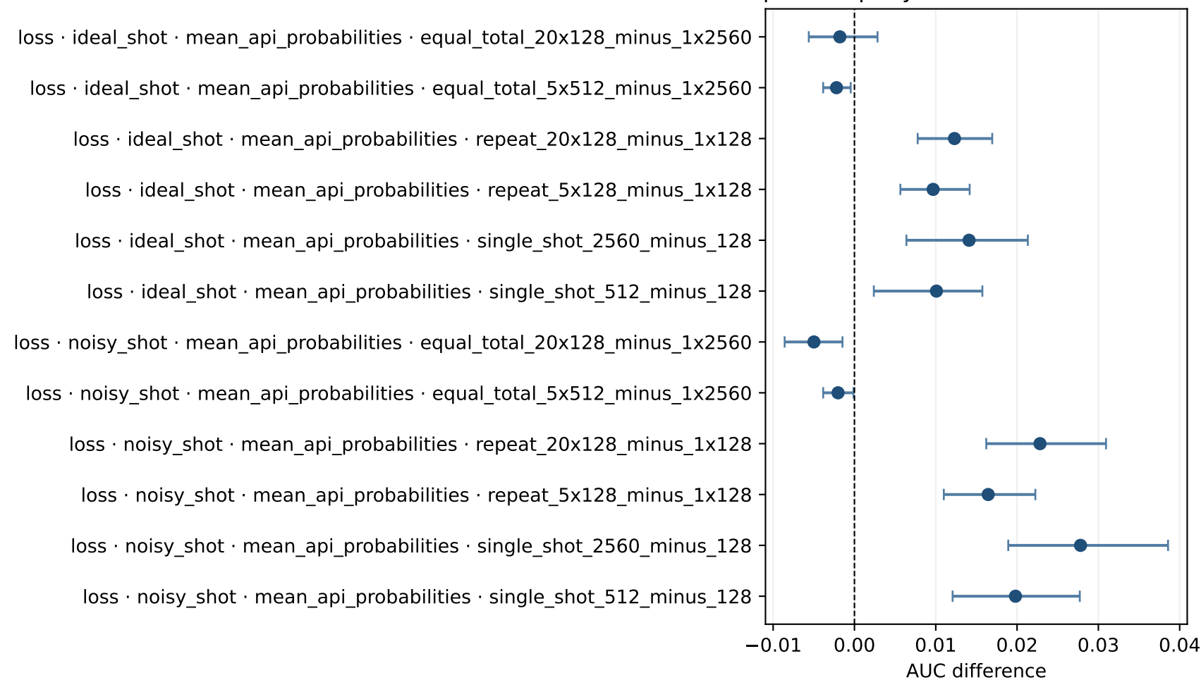
N2 repeated-query and shot-allocation contrasts
