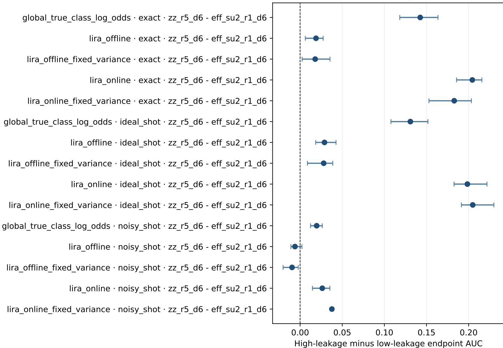
N3 LiRA structural endpoint contrast
