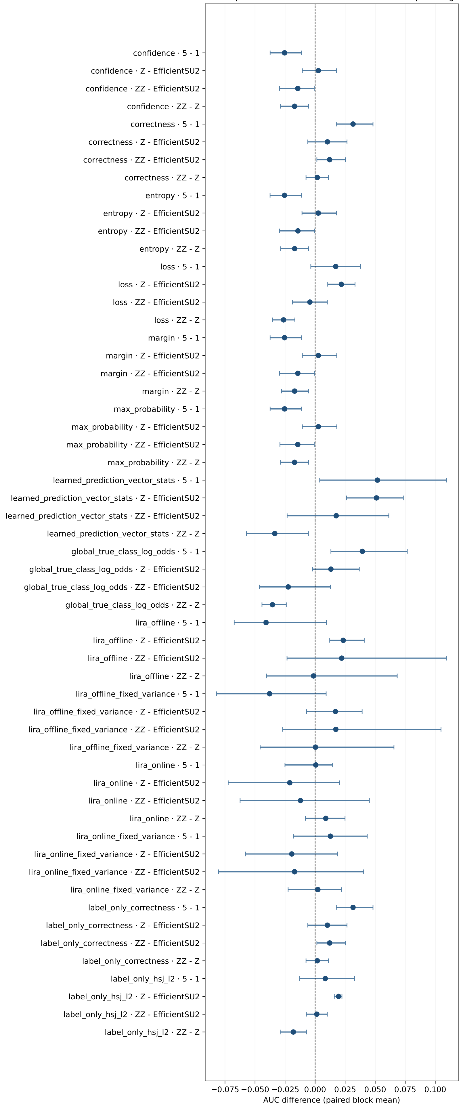
WDBC paired structural effects on membership leakage
