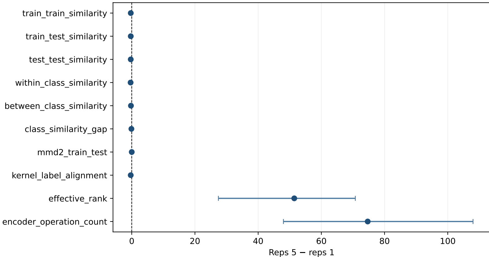
WDBC repetition-induced geometry changes
