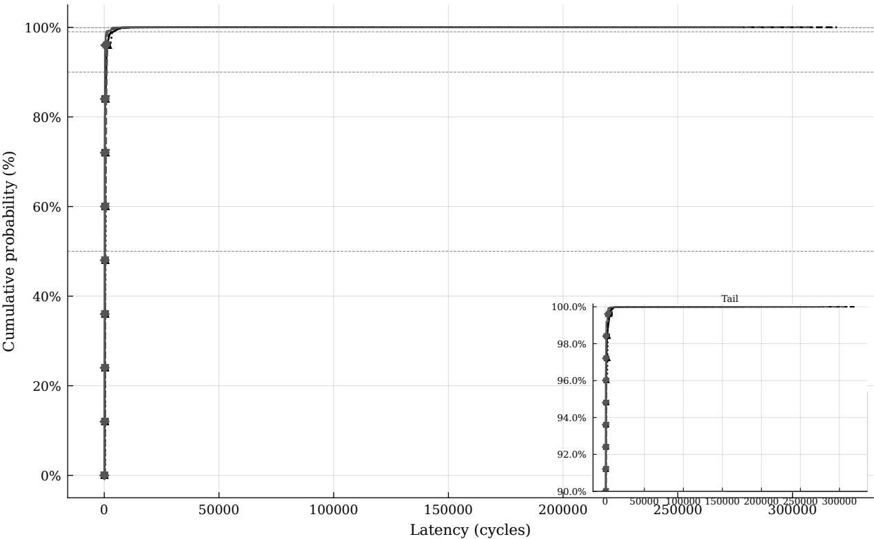
Queue comparison: lightly loaded (enqueue)
