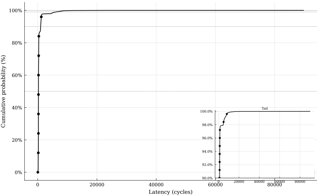
coarse mutex: workload comparison (dequeue)
