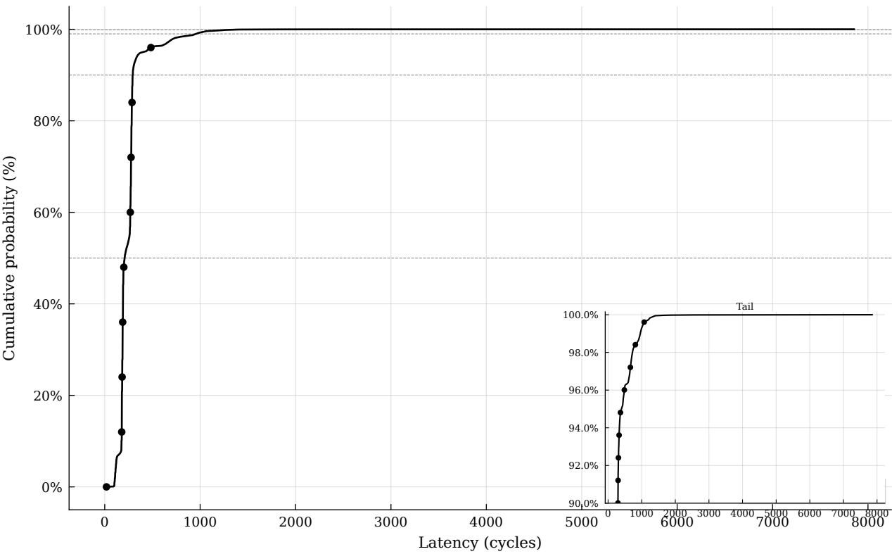
spsc ring: workload comparison (dequeue)
