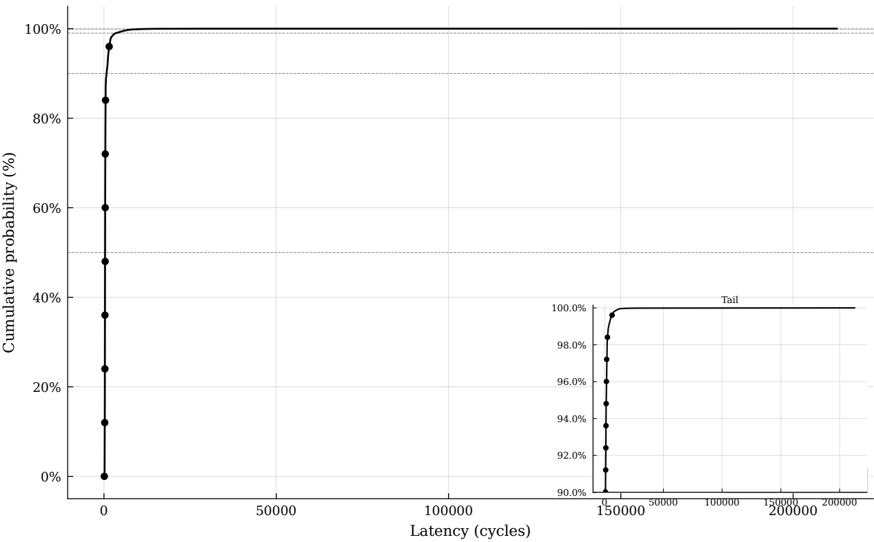
two locks: workload comparison (dequeue)
