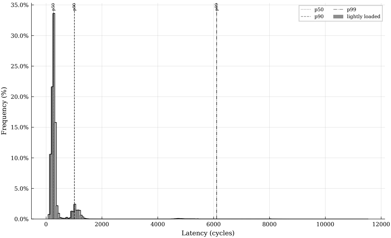
coarse mutex: workload comparison (dequeue)
