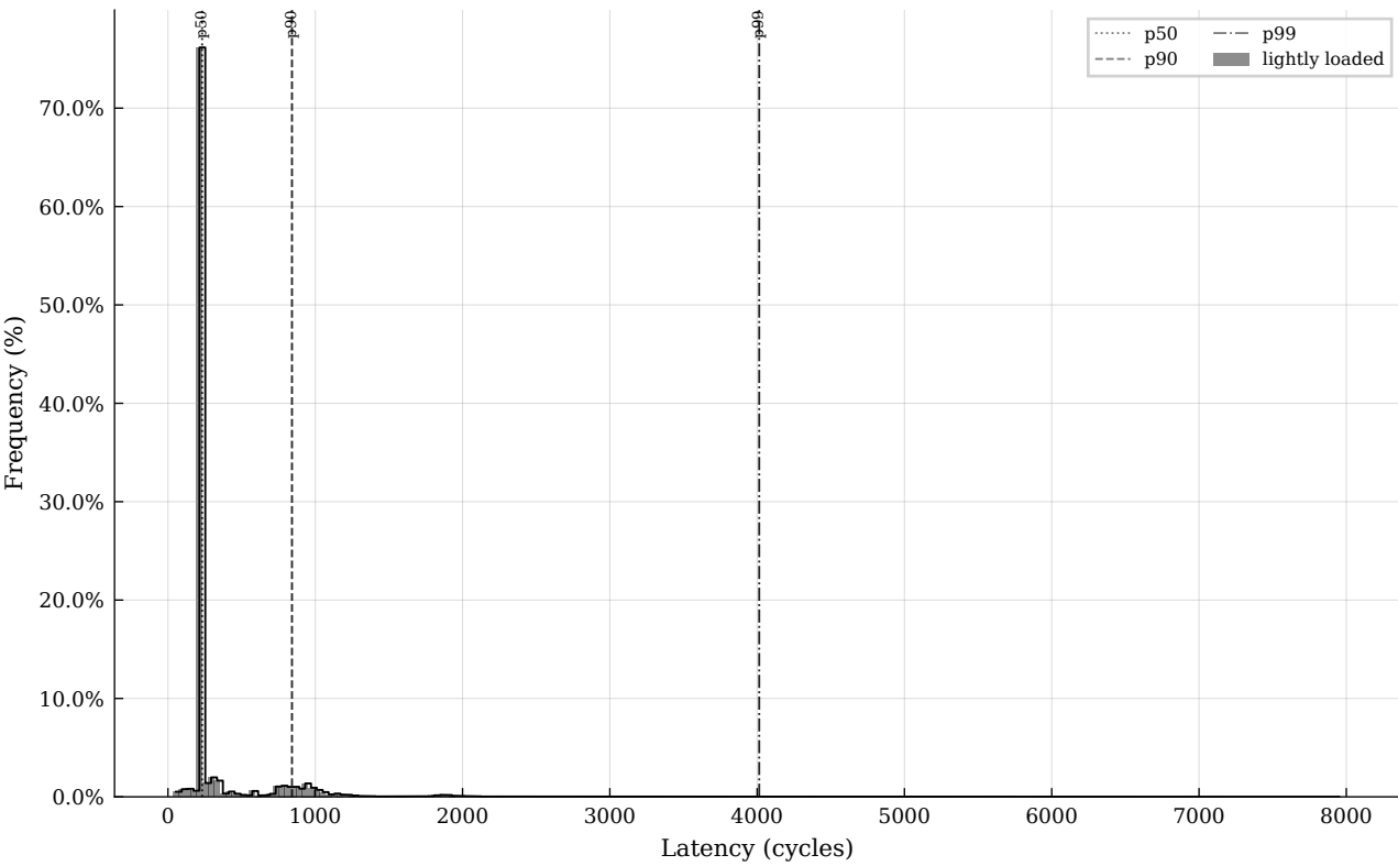
coarse mutex: workload comparison (enqueue)
