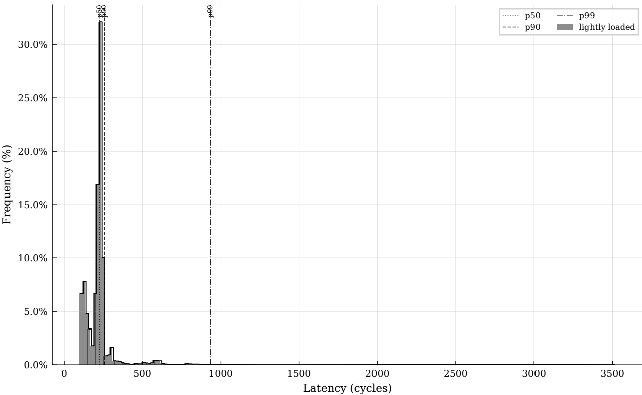
spsc ring: workload comparison (enqueue)
