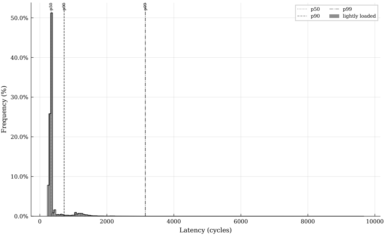
two locks: workload comparison (enqueue)
