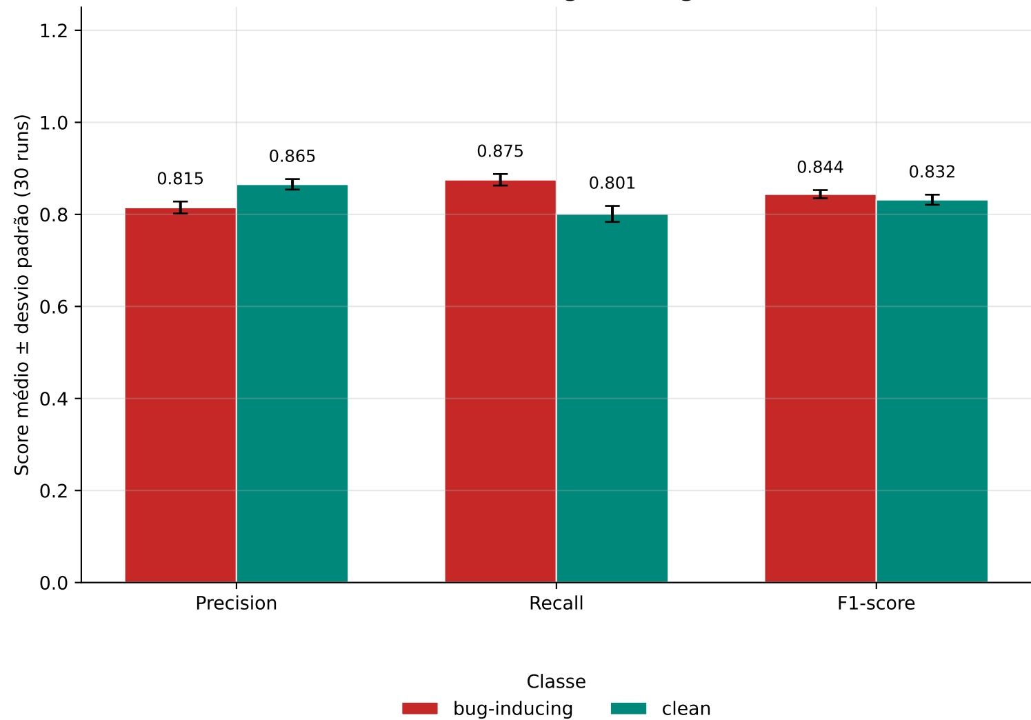
Random Forest — Bug-inducing vs Clean
