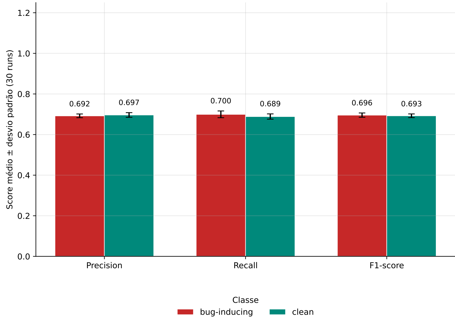
Logistic Regression — Bug-inducing vs Clean
