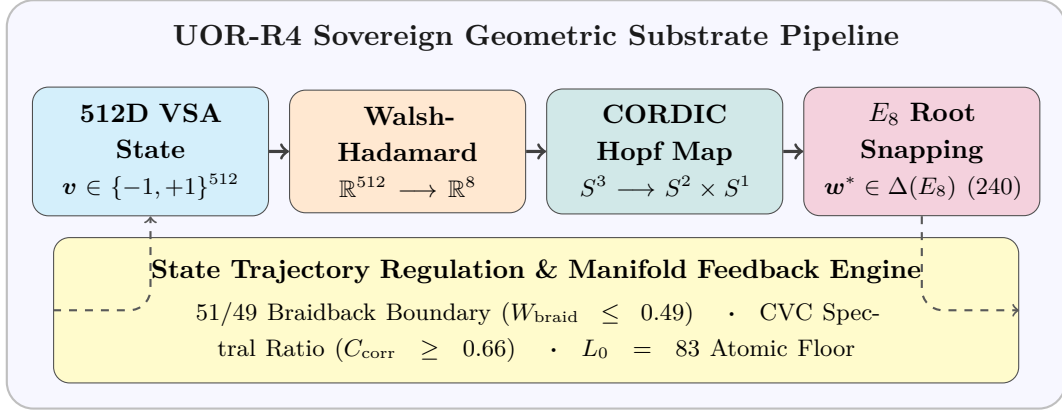
Figure 1: Architectural dataflow of the UOR-R4 deterministic geometric state machine. High-dimensional 512D bipolar VSA states are projected onto an 8D Lie algebraic subspace, routed via 15-iteration CORDIC Hopf fibrations ( S^3 \rightarrow S^2 ), quantized onto the 240 minimal roots of the Gosset E_8 lattice, and stabilized via closed-loop trajectory invariants.
