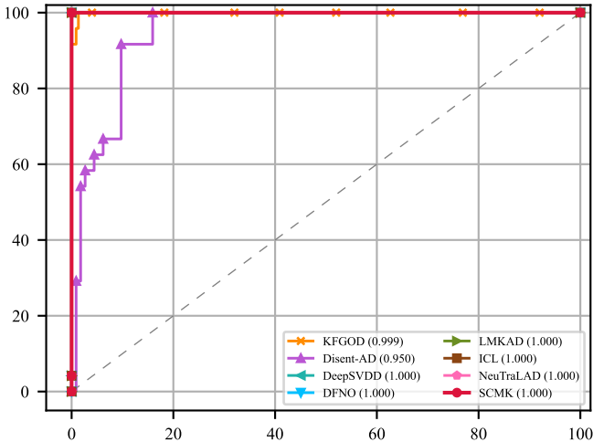
Ionosphere
