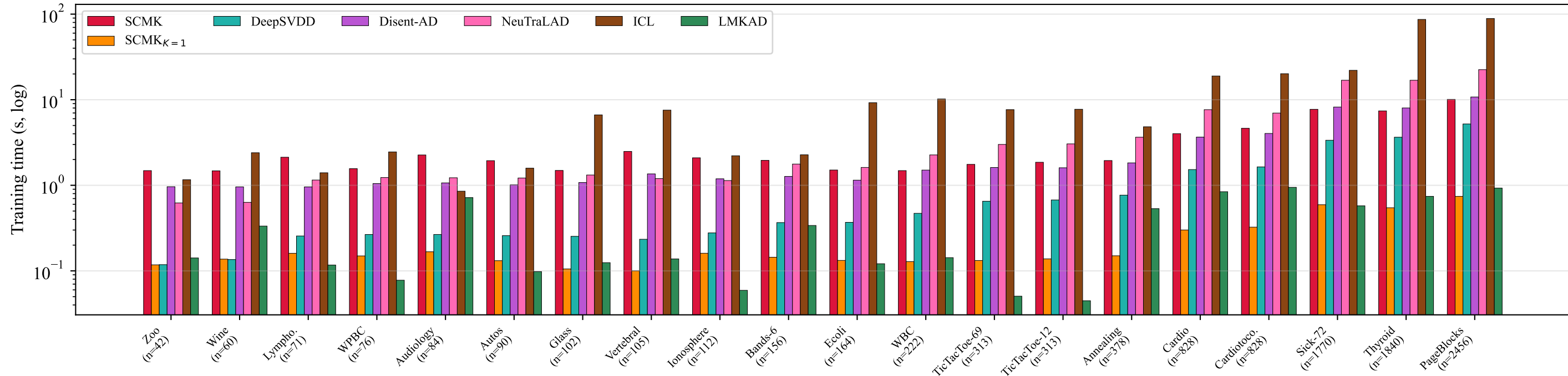
Per-dataset training time (datasets sorted by training-set size n )
