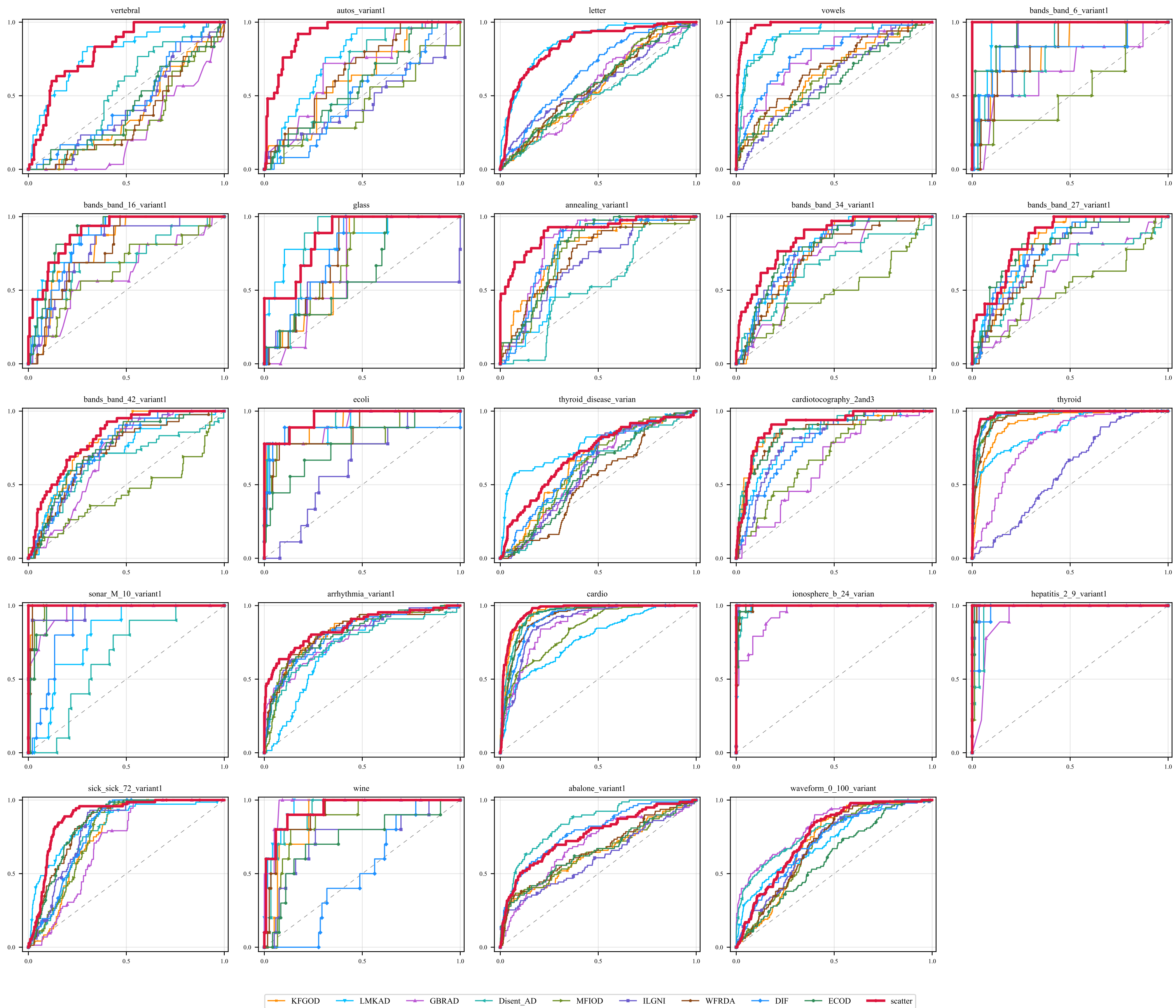
ROC: KFGOD/LMKAD (replacing NGBAD/ROD) + 7 algs vs scatter
