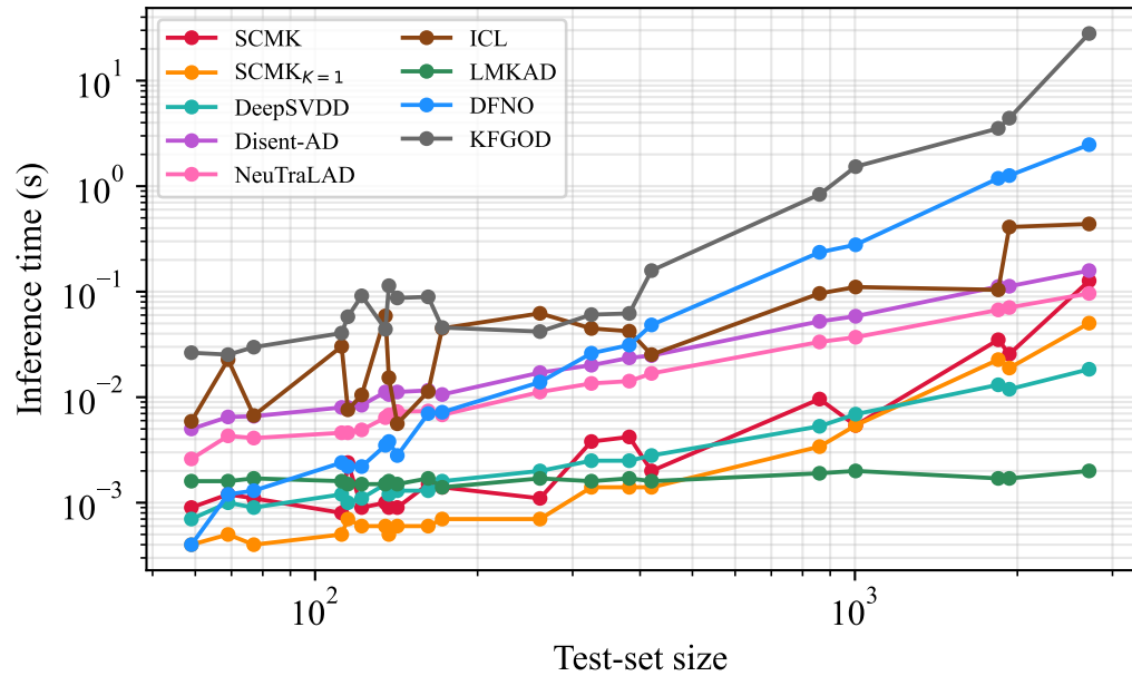
(b) Inference time vs size
