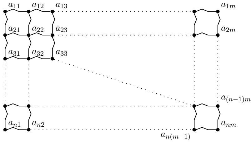
Figure 1: Spring model of a cardiomyocyte
