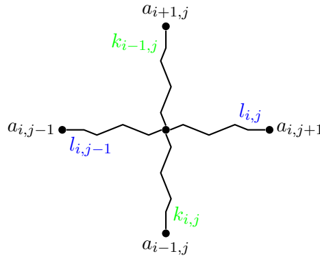
Figure 2: Spring coefficients neighbouring Z-disk a_{i,j} .
