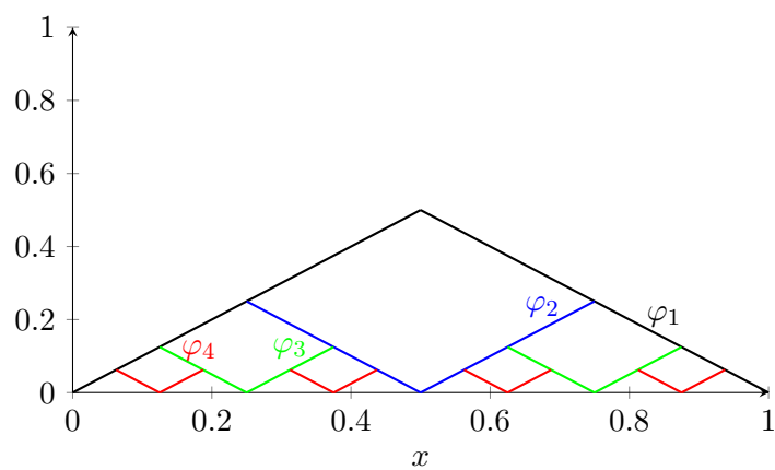
Figure 2.1: Many Lipschitz a.e. solutions.
