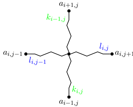
Figure 2: Spring coefficients neighbouring Z-disk a_{i,j} .
