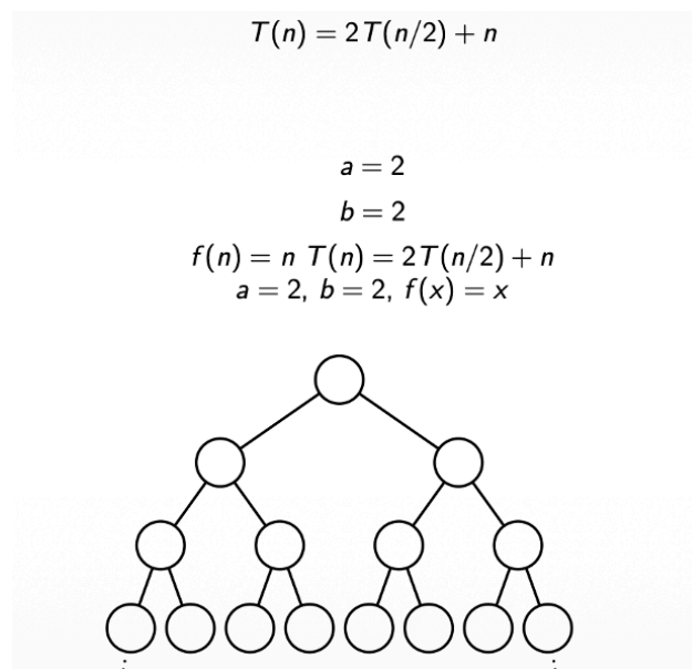
Figur 48: T(n) = 2T\left(\frac{n}{2}\right) + n .
