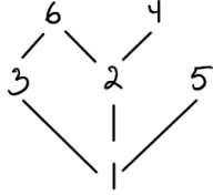
Figur 26: Hasse-diagram for samme delelighedsrelation.
