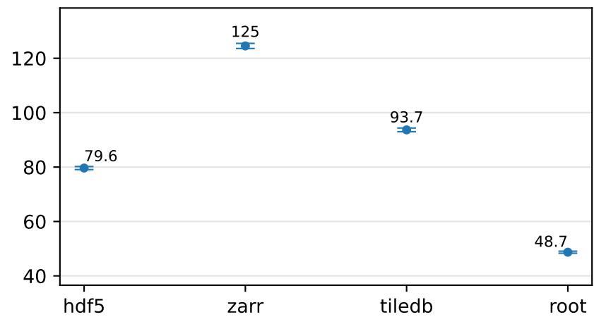
zstd / full
