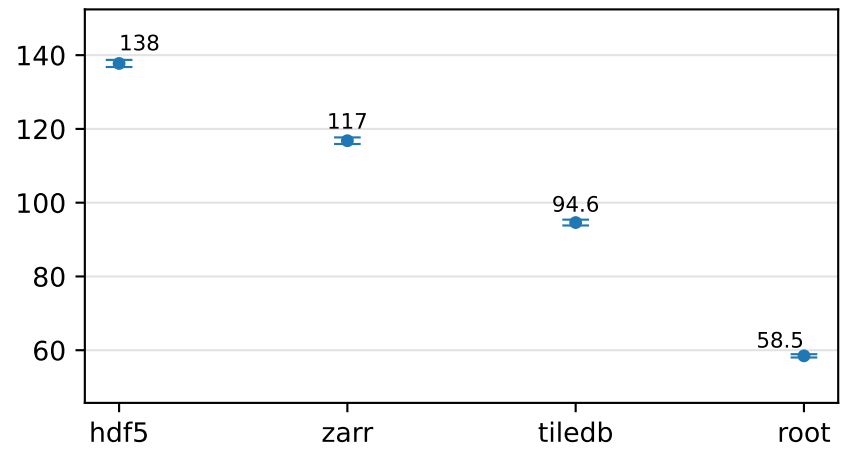
lz4 / full
