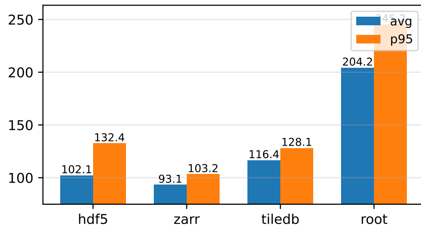
lz4 / full
