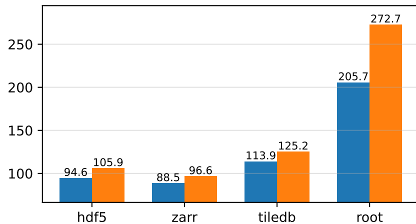
zstd / full
