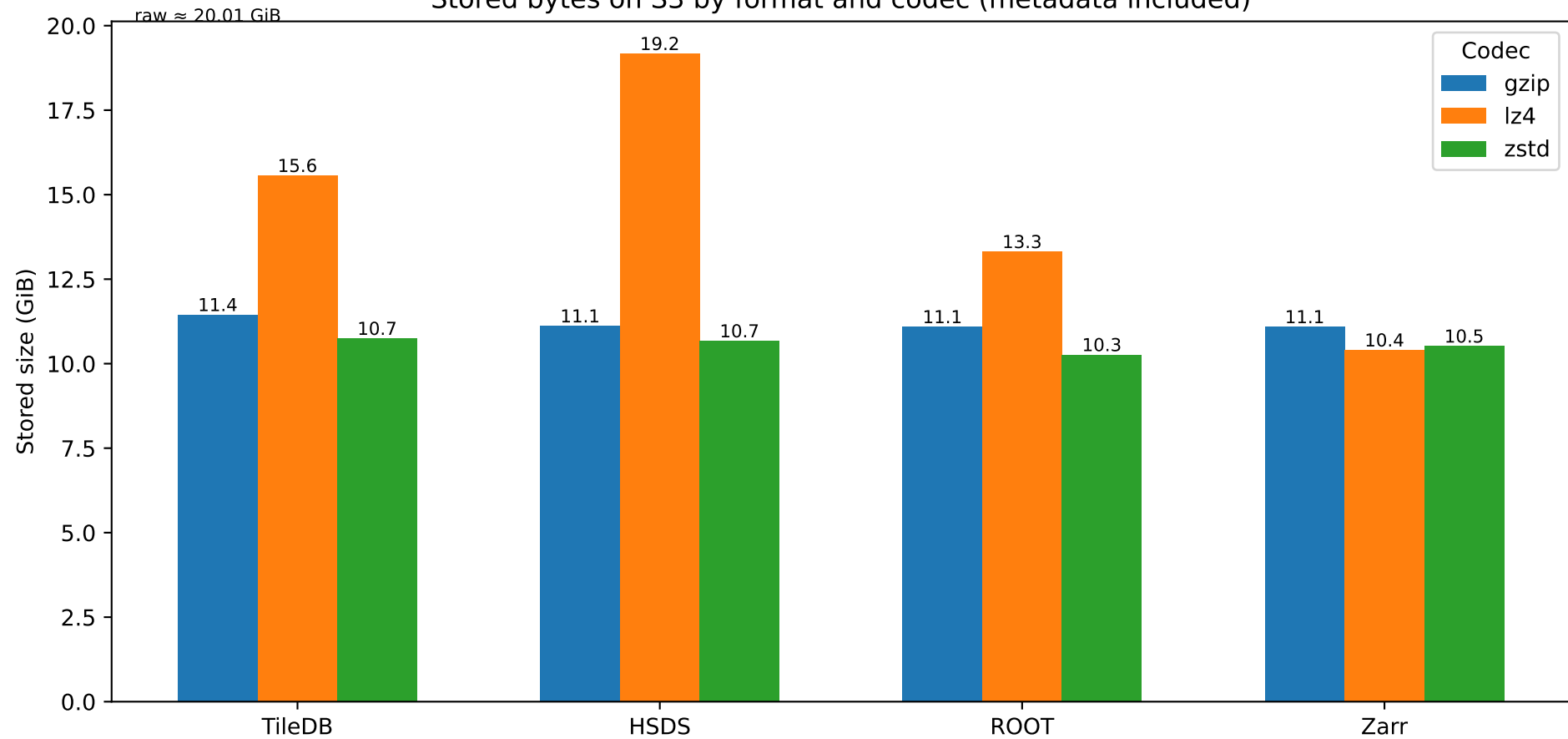
Stored bytes on S3 by format and codec (metadata included)
