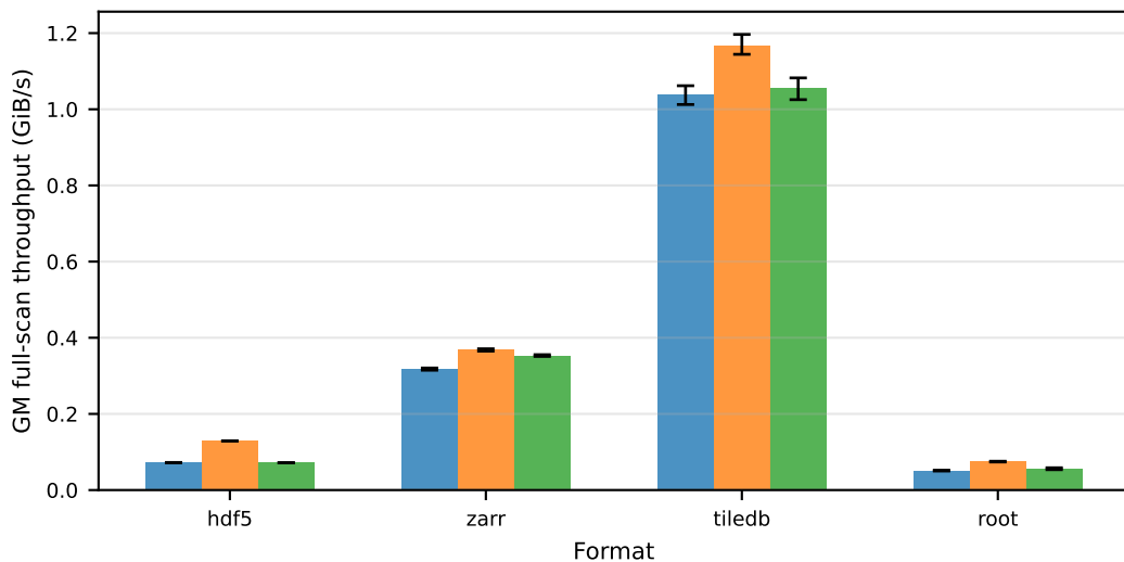
Codec comparison by format — full-scan throughput
