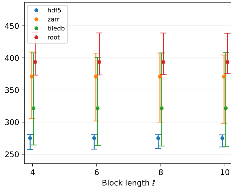
Tail sensitivity (HD p95) — slice: effect of block length
