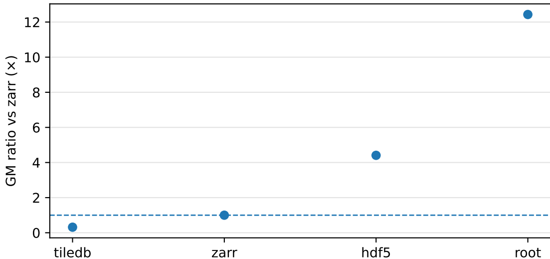
full — gzip: Descriptive GM ratios (session-conditional)
