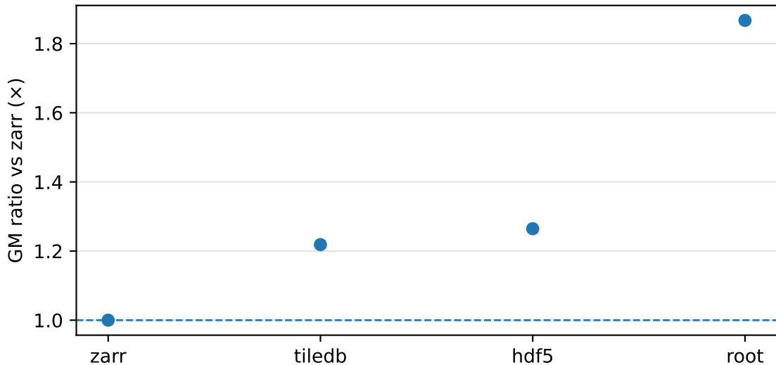
slice — lz4: Descriptive GM ratios (session-conditional)
