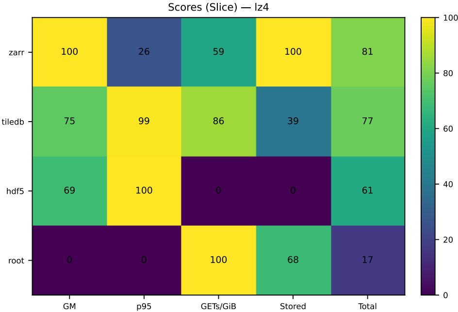
Figure A.25: Slice/lz4: normalized scores.
