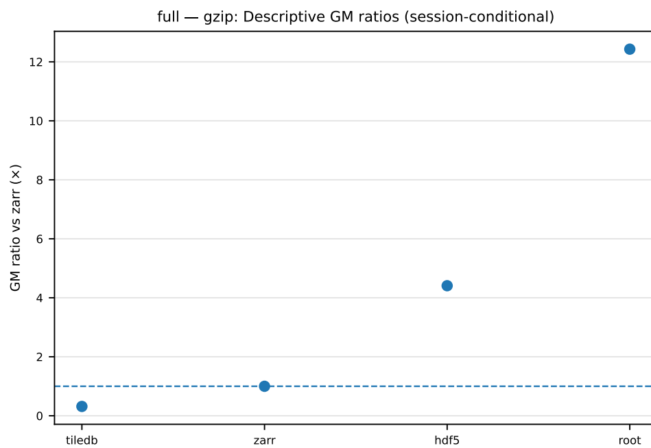
Figure A.32: gzip/full : descriptive GM time ratios vs Zarr (session-conditional).
