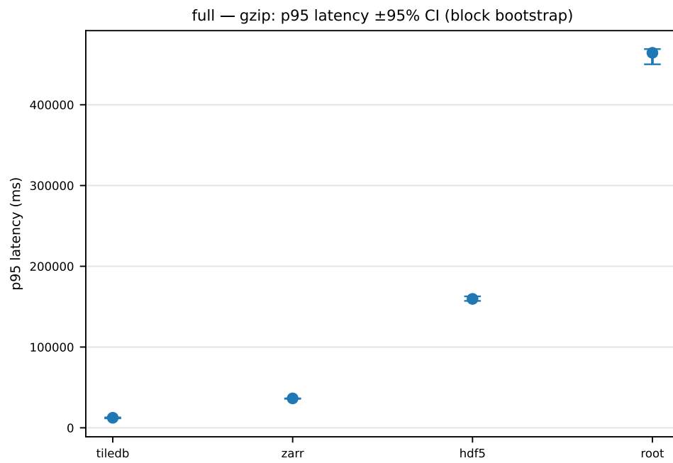
Figure A.31: gzip/full : p_{95} time with dependence-robust 95% CIs.
