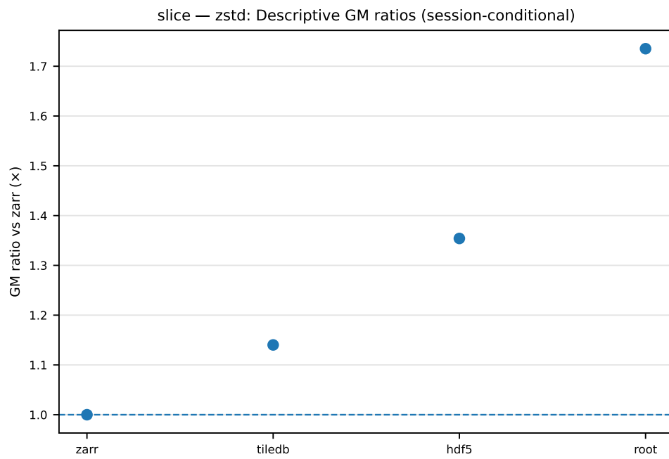
Figure A.19: zstd/slice : descriptive GM time ratios vs Zarr (session-conditional).
