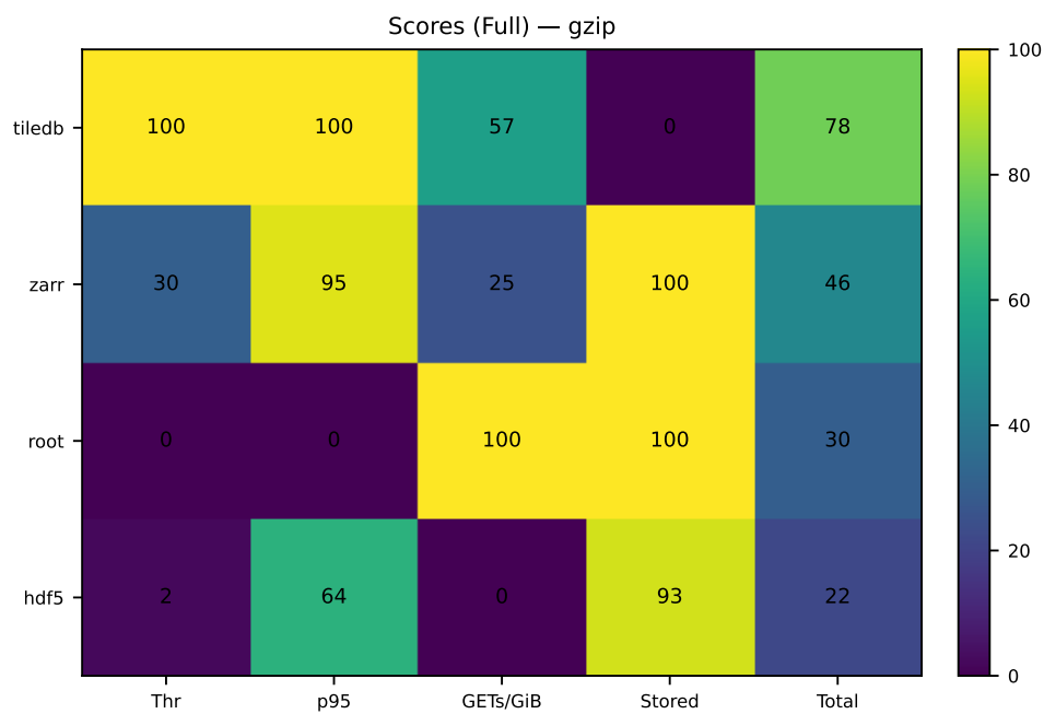
Figure A.27: Full/gzip: normalized scores.
