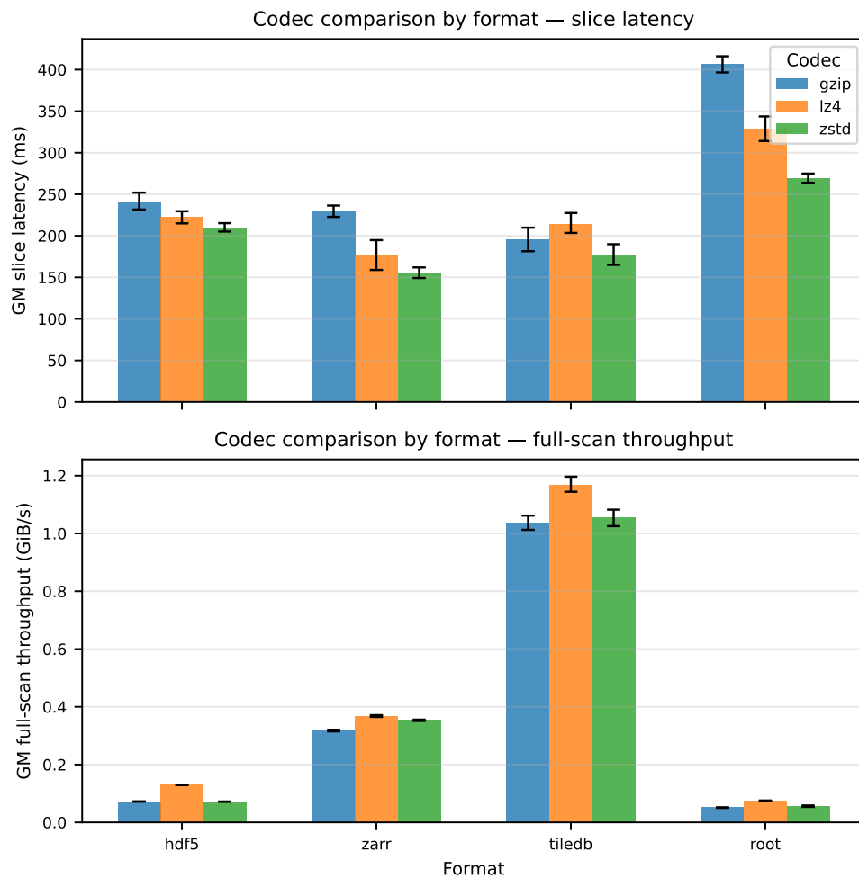
Figure 5.5: Codec comparison by format. Top: GM slice latency (ms); bottom: transferred-byte GM full-scan throughput (GiB/s). Bars are grouped by format with one bar per codec (gzip, LZ4, zstd); error bars show dependence-robust 95% CIs.
