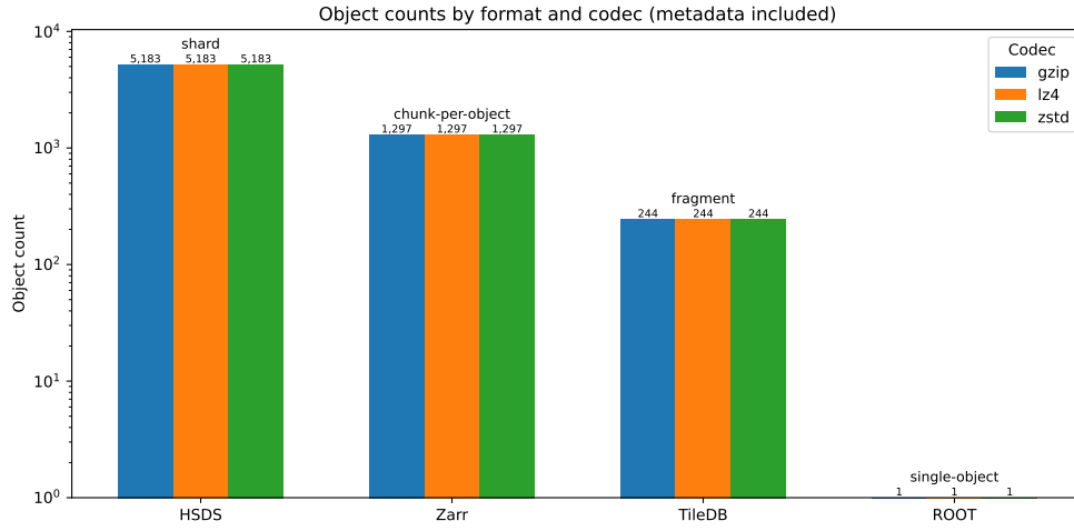
Figure 5.3: Object counts by format and codec with annotated layout type (log-scale y-axis). Counts include data and metadata objects.
