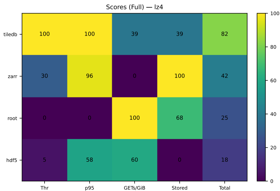
Figure A.28: Full/lz4: normalized scores.
