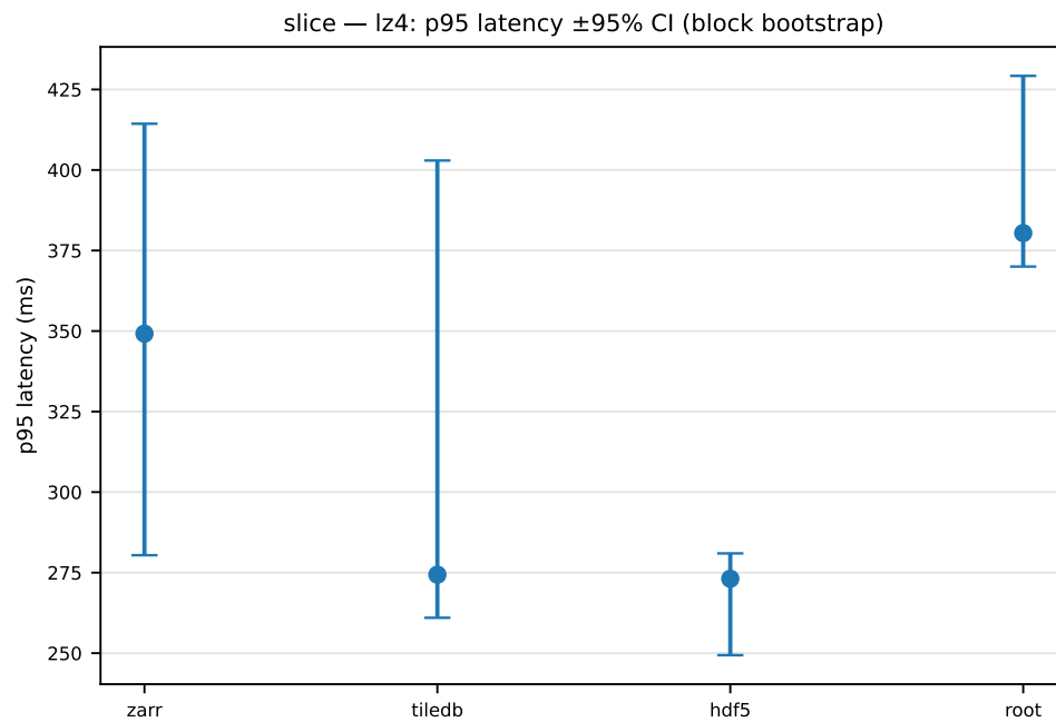
Figure A.15: \text{1 z 4/slice} : p_{95} latency with dependence-robust 95% CIs.
