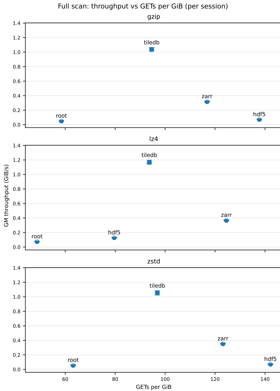
Figure 5.7: Full scan: transferred-byte GM throughput (GiB/s, dependence-robust CI from time) versus GETs per GiB by format and codec. Points are per session; no inference.
