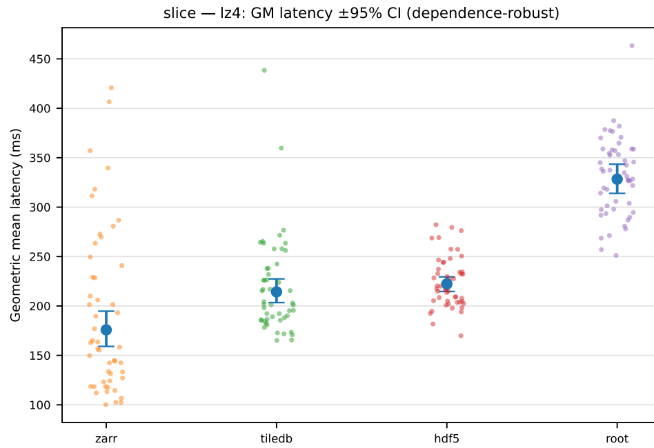
Figure A.14: \text{1 z 4/slice} : geometric mean latency with dependence-robust 95% CIs.
