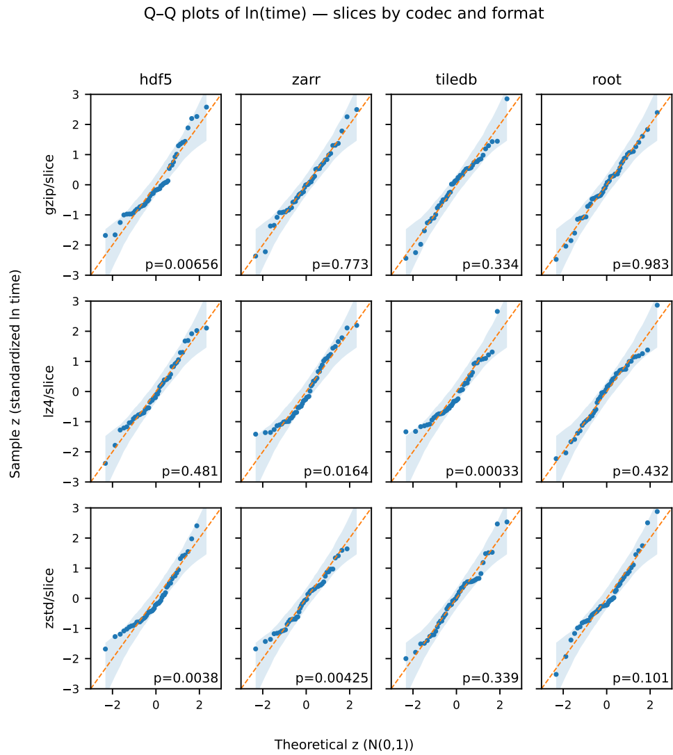
Figure A.1: Q-Q plots of \ln(\text{time}) for slice workloads. Rows: codecs {gzip, lz4, zstd}. Columns: formats {HDF5/HSDS, Zarr, TileDB, ROOT/TTTree}. Shaded band is a 95% pointwise envelope; per-panel Shapiro p shown.
