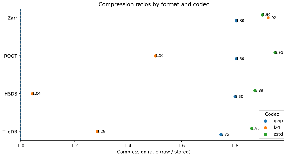
Figure 5.2: Compression ratios R_{f,c} = B_{\text{raw}}/B_{f,c}^{\text{stored}} for the same format–codec totals (higher is better). Minor between-format differences at fixed codec are consistent with additional layout metadata.
