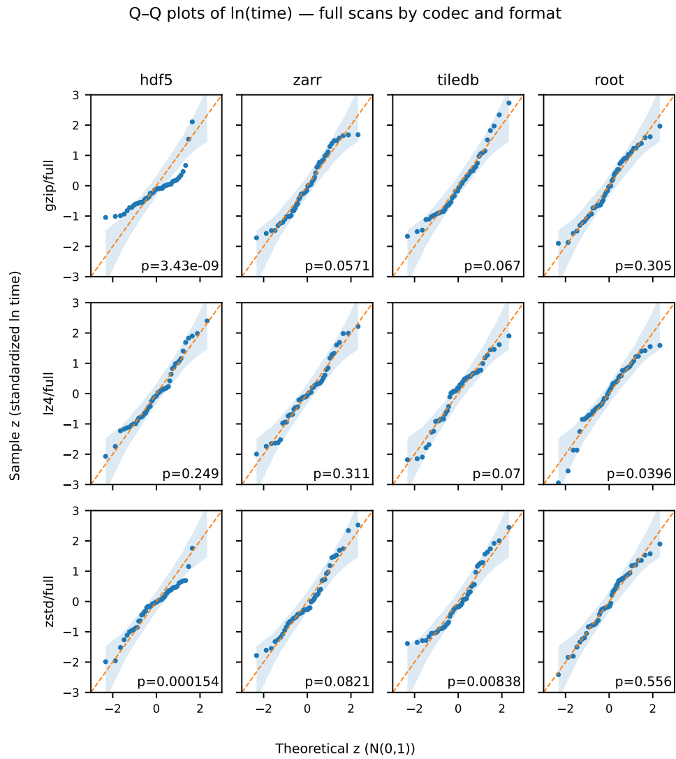
Figure A.2: Q-Q plots of \ln(\text{time}) for full-scan workloads. Rows: codecs {gzip, lz4, zstd}. Columns: formats {HDF5/HSDS, Zarr, TileDB, ROOT/Tree}. Shaded band is a 95% pointwise envelope; per-panel Shapiro p shown.
