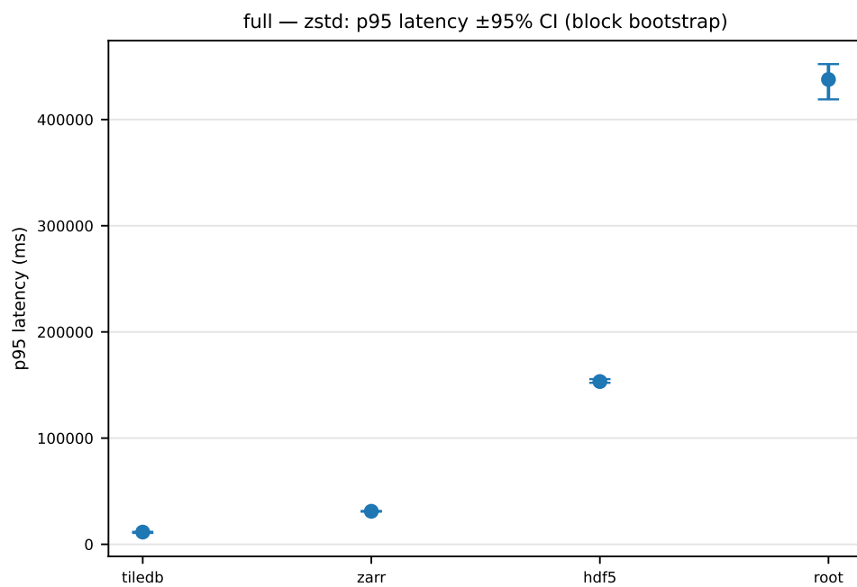
Figure A.37: zstd/full : p_{95} time with dependence-robust 95% CIs.
