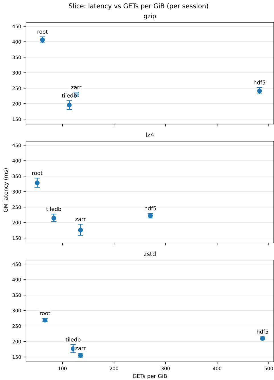
Figure 5.6: Slice: GM latency (ms, dependence-robust CI) versus GETs per GiB by format and codec. Points are per session; no inference.
