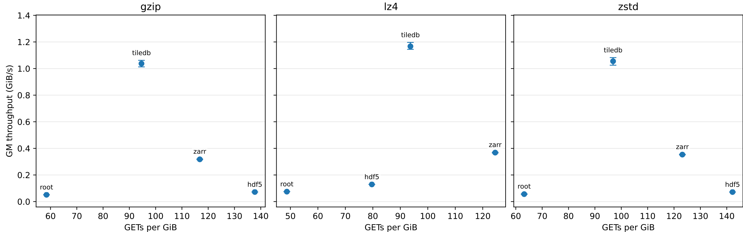
Full scan: throughput vs GETs per GiB (per session)
