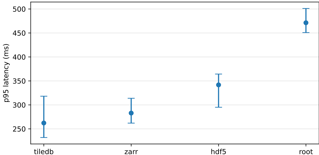
slice — gzip: p95 latency \pm 95% CI (block bootstrap)
