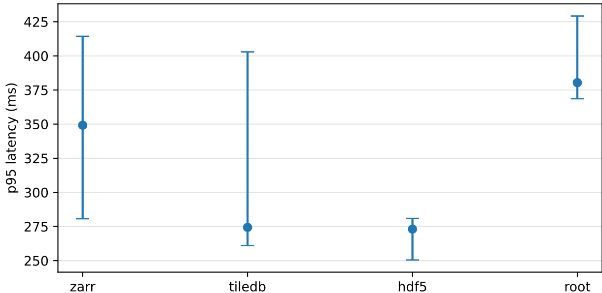
slice — lz4: p95 latency \pm 95% CI (block bootstrap)
