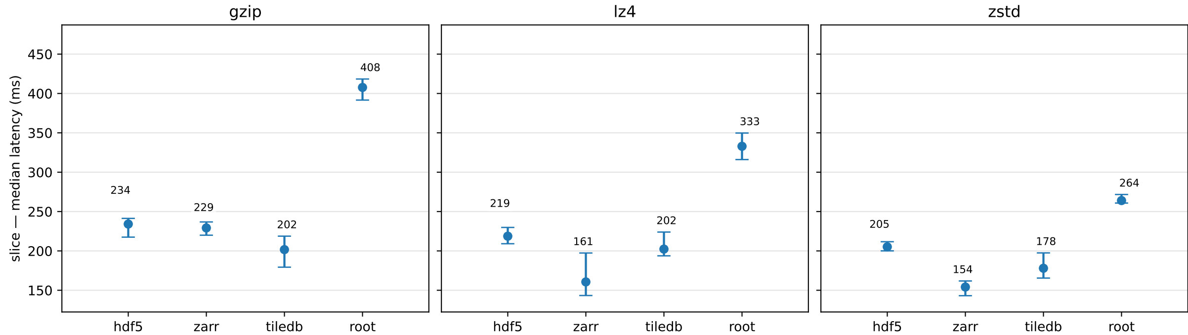
Median latency \pm 95% CI (MBB) — slice
