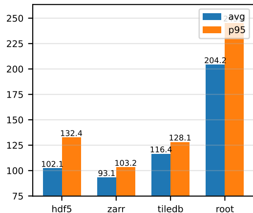
lz4 / full
