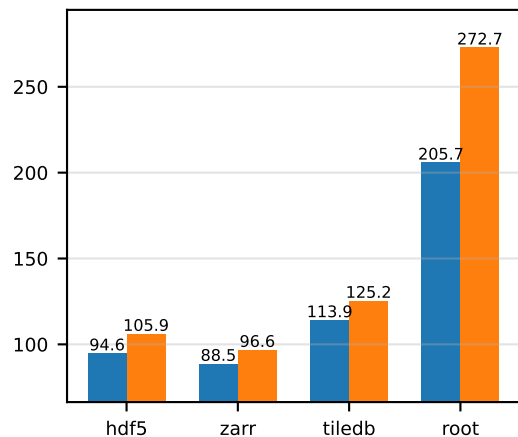
zstd / full
