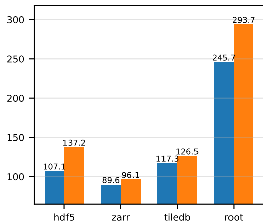
zstd / full
